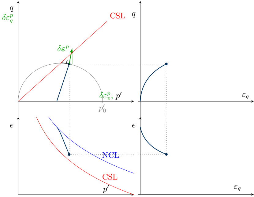
Modified Cam Clay Model (Roscoe & Burland, 1968): Drained triaxial test of normally consolidated clay
