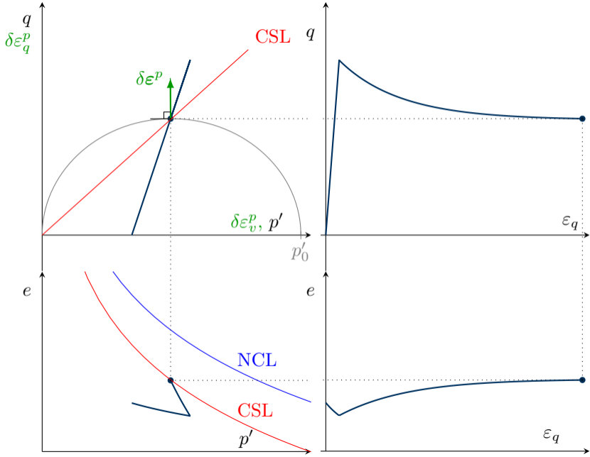
Modified Cam Clay Model (Roscoe & Burland, 1968): Drained triaxial test of highly overconsolidated clay
