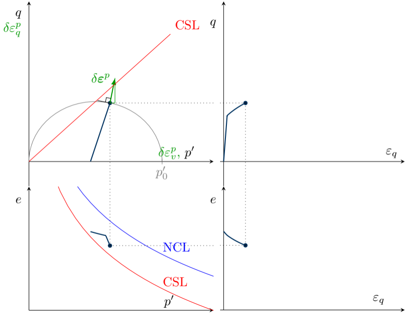
Modified Cam Clay Model (Roscoe & Burland, 1968): Drained triaxial test of slightly overconsolidated clay
